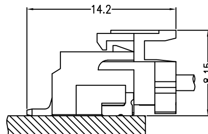
Assembly Layout
