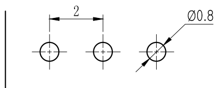
P. C. B LAYOUT
