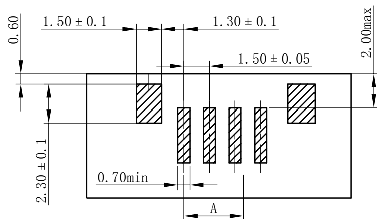
PCB LAYOUT
